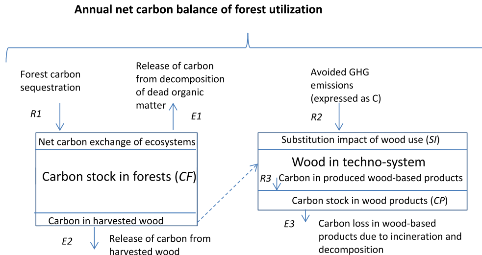
Fig. 1. Schematic description of carbon emissions ( E ) and removals ( R ) causing annual net carbon balance of forest utilization. \Delta CF = R1 - E1 - E2 , \Delta CP = R3 - E3 and SI = R2 when E s and R s are measured as positive values.
